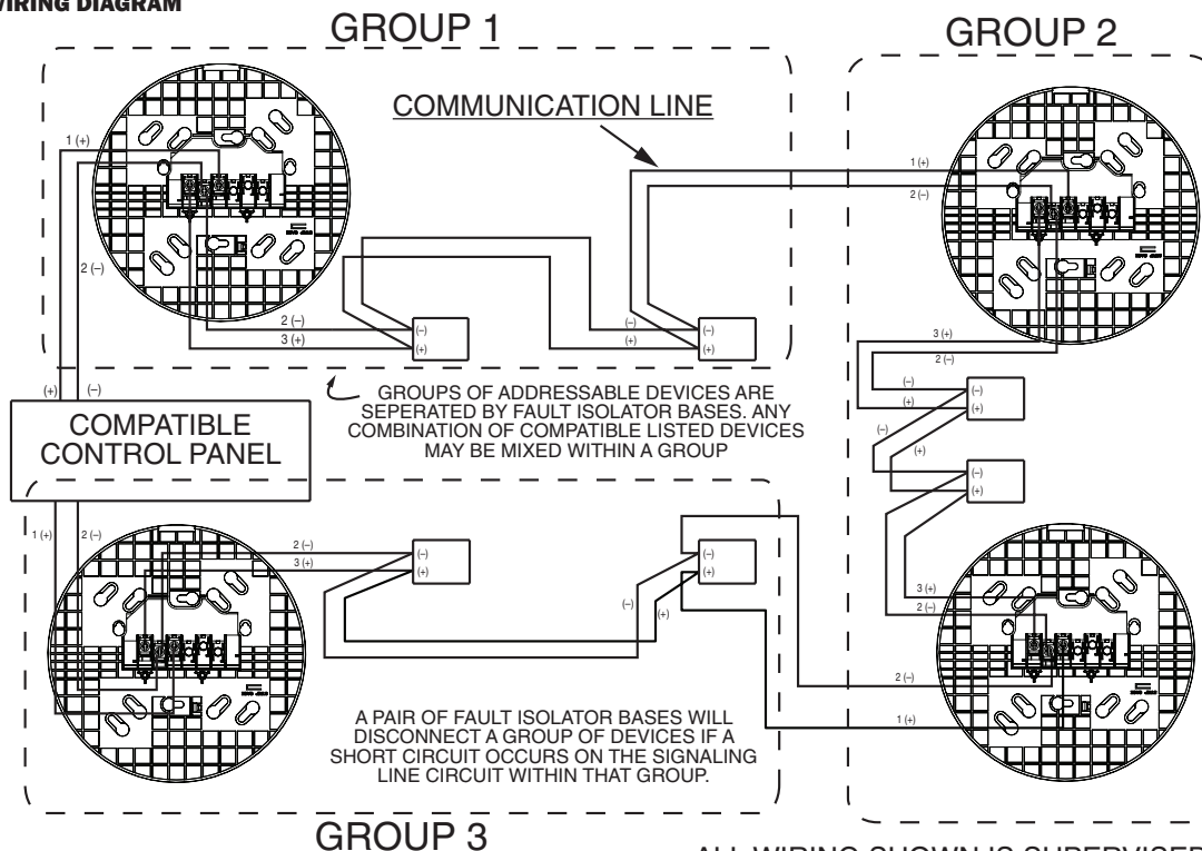
FIGURE 4. WIRING DIAGRAM
