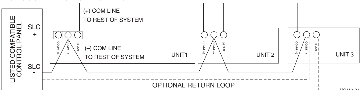
FIGURE 6. SYSTEM WIRING DIAGRAM FOR DNRECL:
