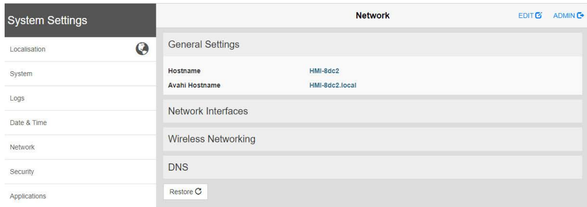
Fig. 13 Network settings
