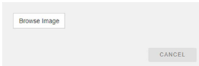
Fig. 38 Browse Image
