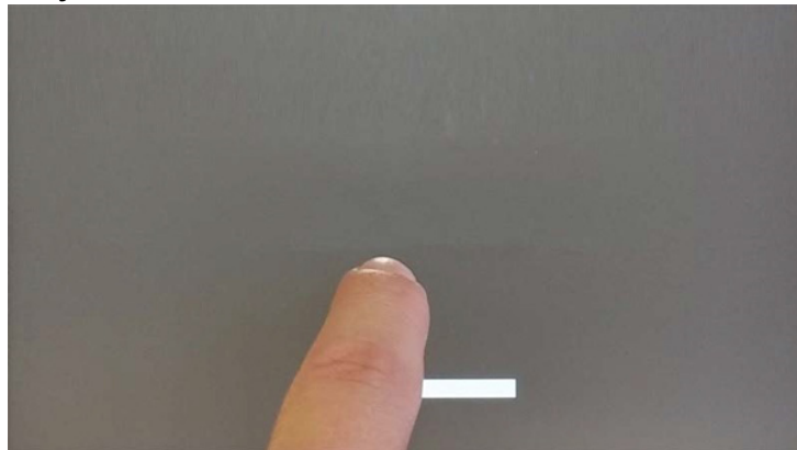
Fig. 33 System Settings
