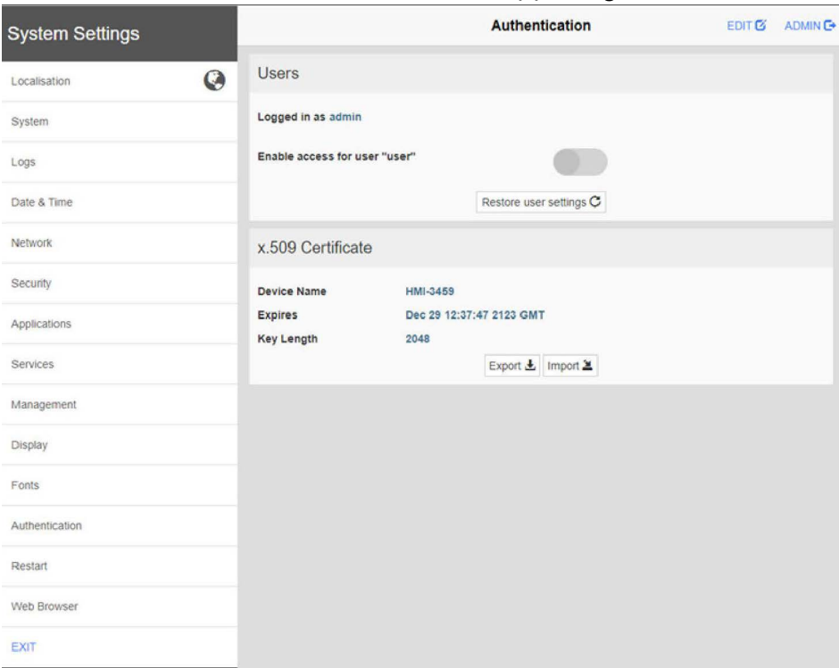
Fig. 25 System settings
