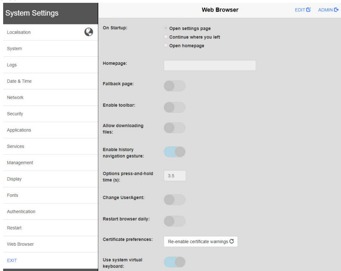
Fig. 10 System Settings
