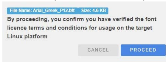
Fig. 22 Selected font
