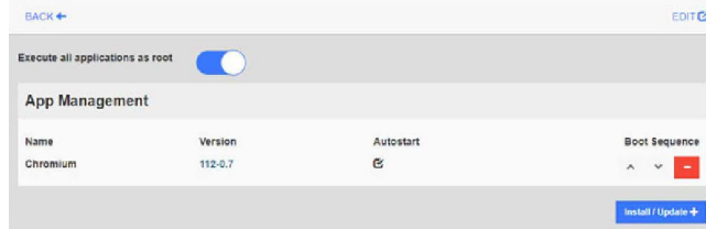
Fig. 37 App Management
