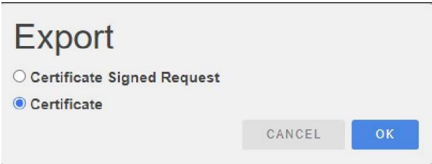
Fig. 24 Export button
