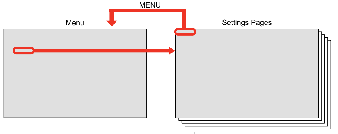
Fig. 11 Settings page
