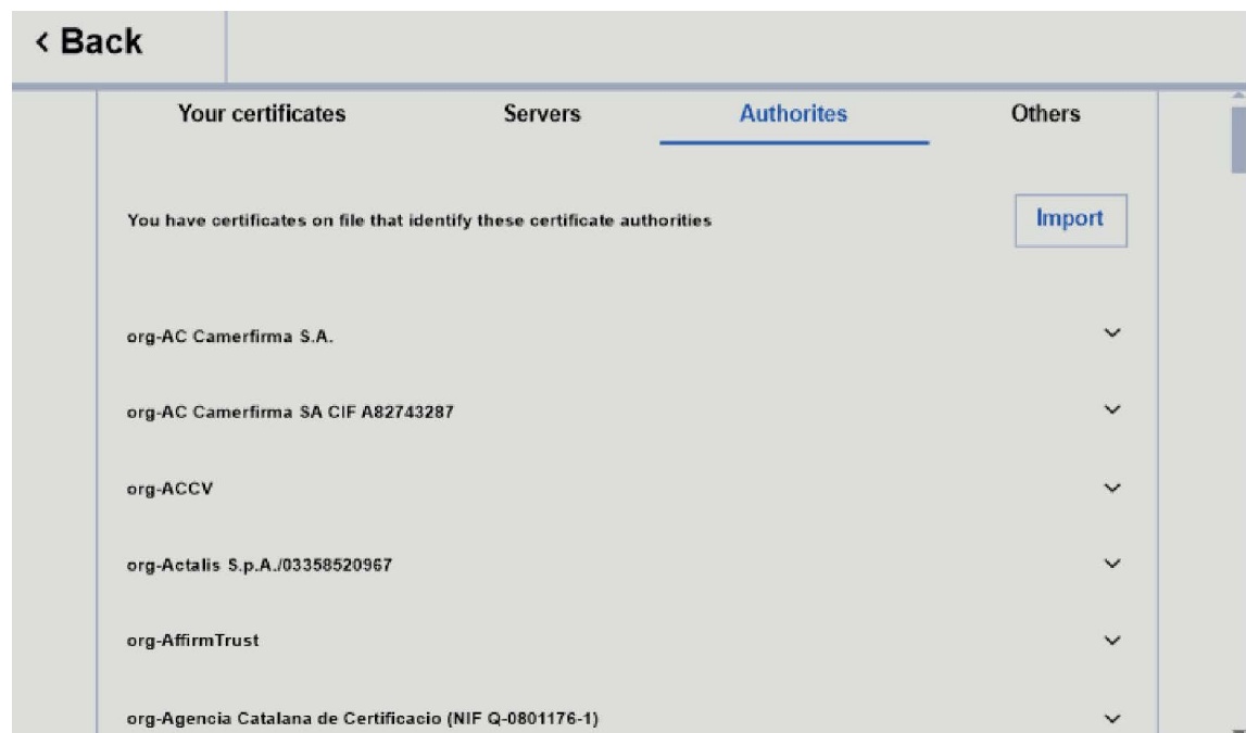
Fig. 45 Authorities
