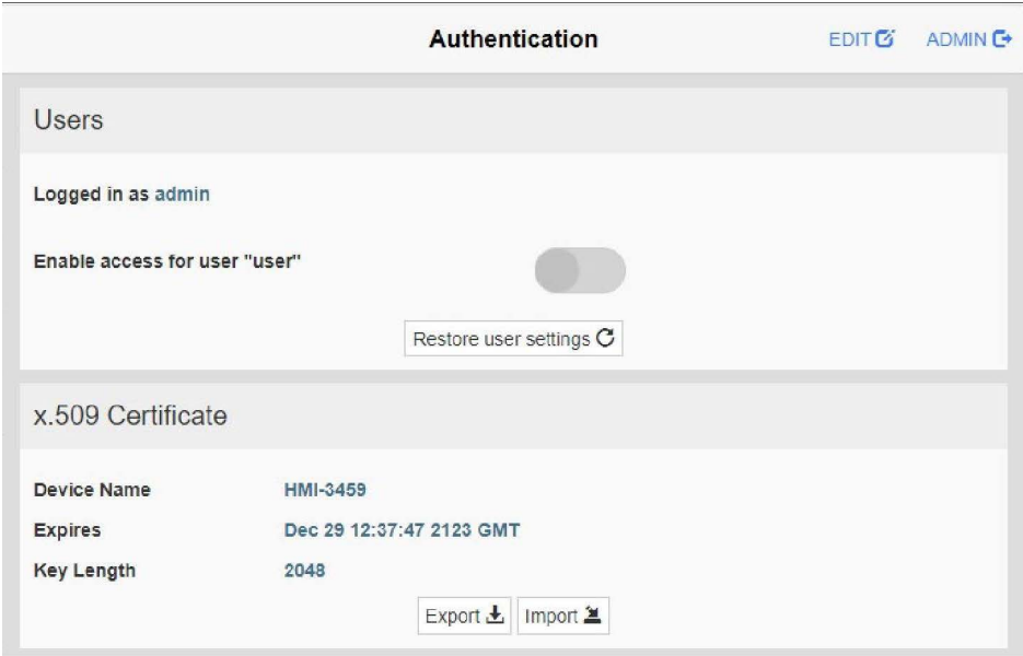
Fig. 23 Authentication
