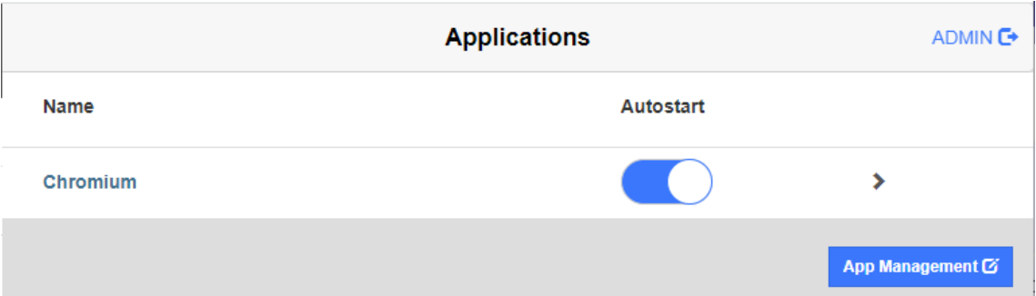
Fig. 18 Applications
