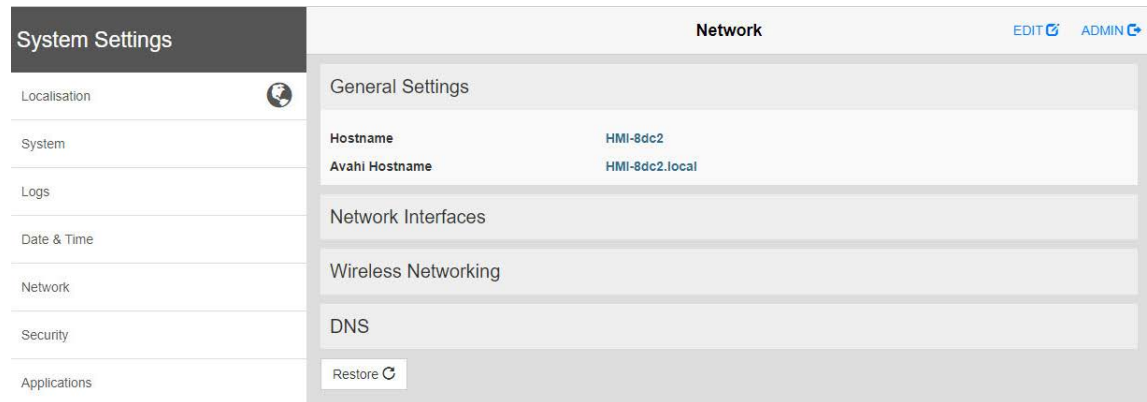
Fig. 13 Network settings
