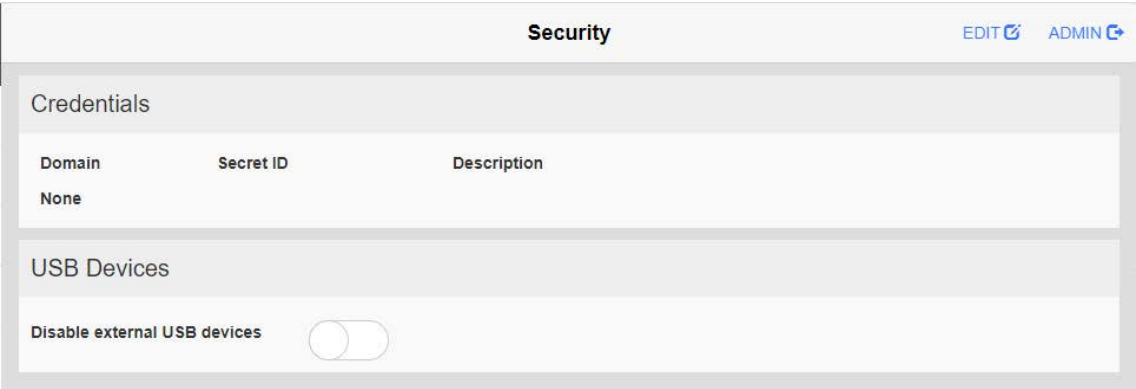
Fig. 17 Security Page
