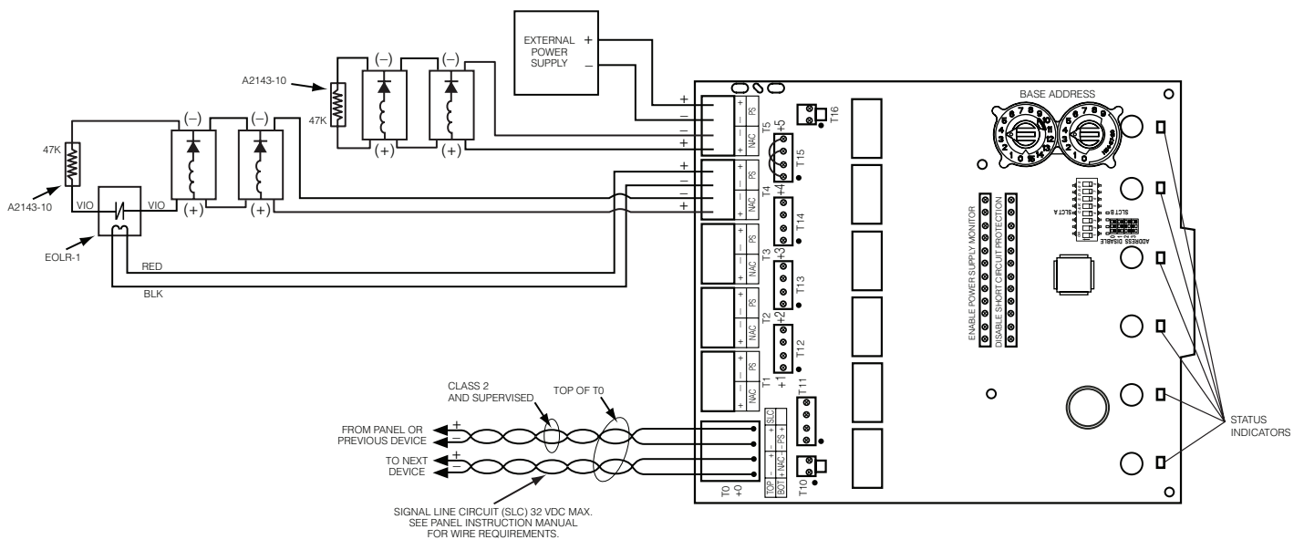
FIGURE 10: EXAMPLE OF CLASS B NAC CONFIGURATION WITH A SINGLE SUPPLY SHARED BY 2 NACS
