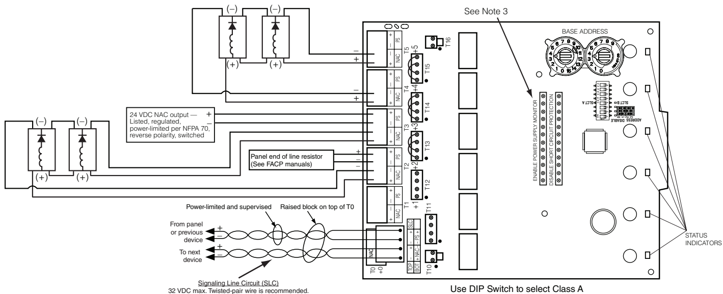
FIGURE 12: EXAMPLE OF CLASS A NAC CONFIGURATION WITH A SINGLE SUPPLY SHARED BY 2 NACS
