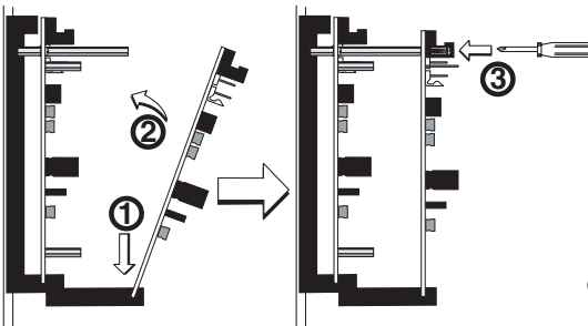
FIGURE 6B: INSTALLATION OF CMF-300-6 MODULE IN FRONT CHASSIS POSITION
