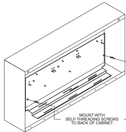
FIGURE 4: MOUNTING THE CH-6 CHASSIS
