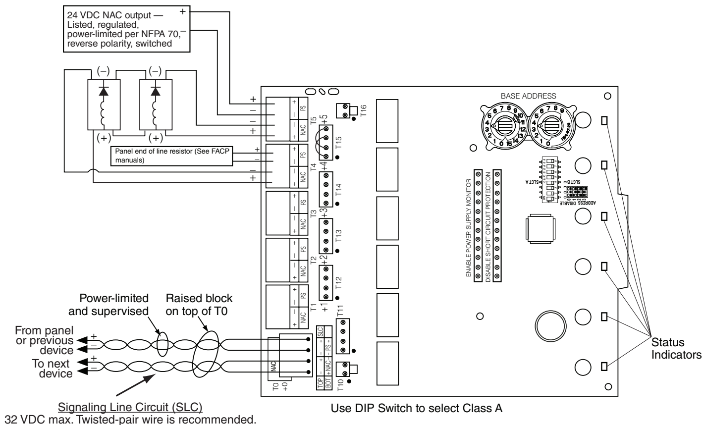
FIGURE 11: EXAMPLE OF CLASS A NAC CONFIGURATION WITH A SINGLE SUPPLY DEDICATED TO A SINGLE NAC
