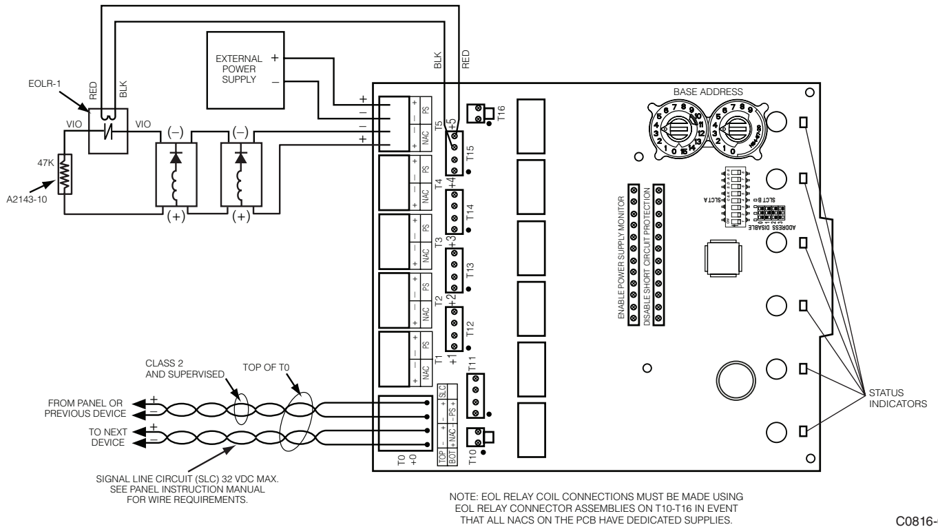
FIGURE 10: EXAMPLE OF CLASS B NAC CONFIGURATION WITH A SINGLE SUPPLY SHARED BY 2 NACS
