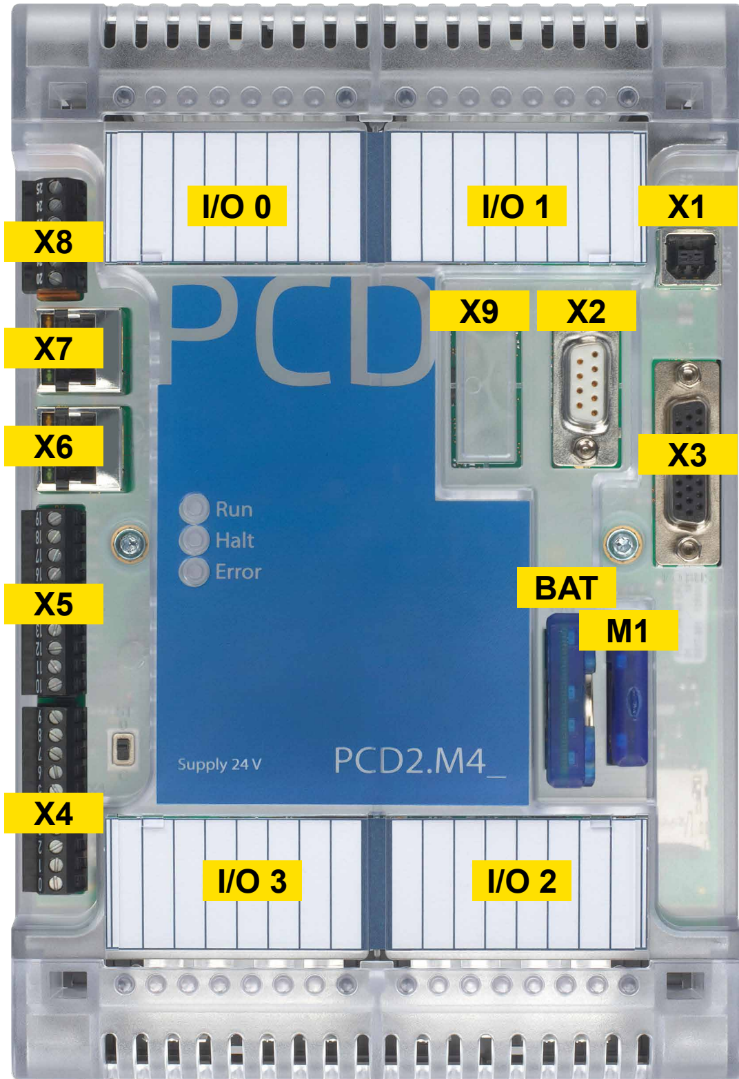
PCD2.M4560
