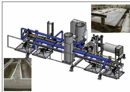
Multiple burner tundish dry out lining and preheating.
