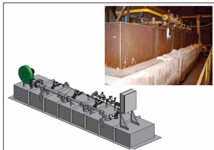
Multiple burner launder dry out lining and preheating.
