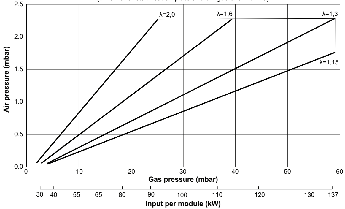
Window of operations of Ratio Star burner for natural gas (Hs = 40 MJ/Nm 3 ) (dP air over stabilisation plate and dP gas over nozzle)
