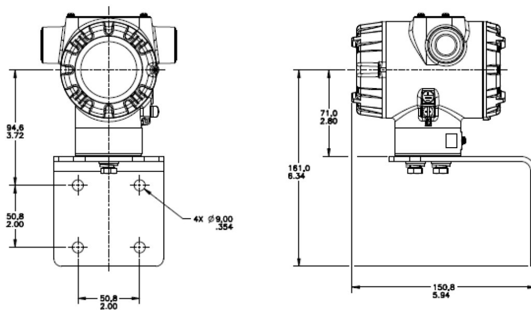
Figure 4 – STT750 housing - Horizontal Wall Mounting
