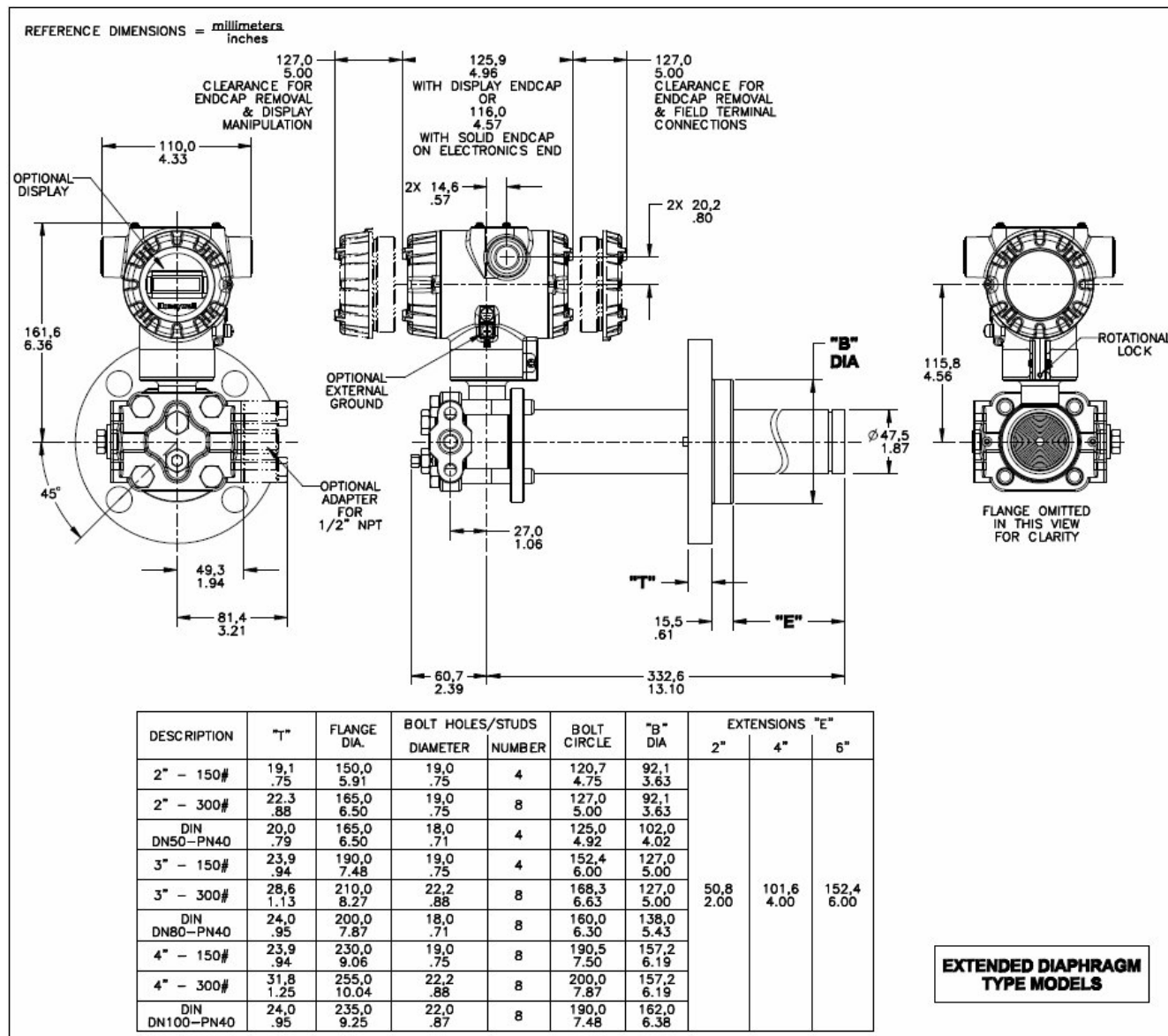
Figure 5 – Typical mounting dimensions for extended diaphragm type models STF724 and STF732.
