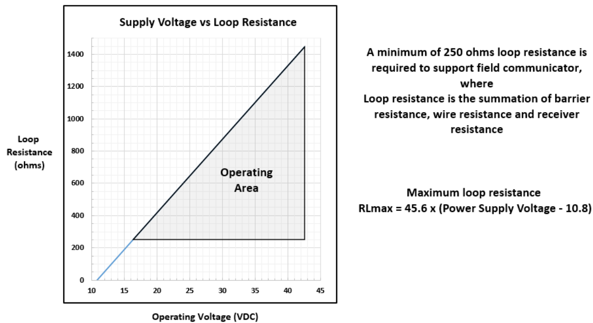
Figure 2 - Supply voltage and loop resistance chart & calculations
