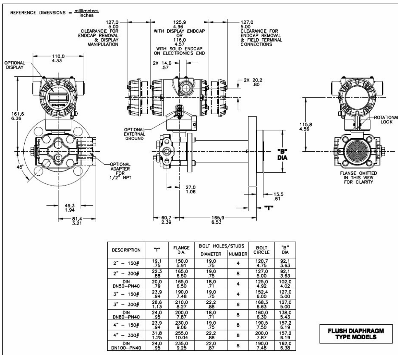
Figure 4 – Typical mounting dimensions for flush diaphragm type models STF724 and STF732.
