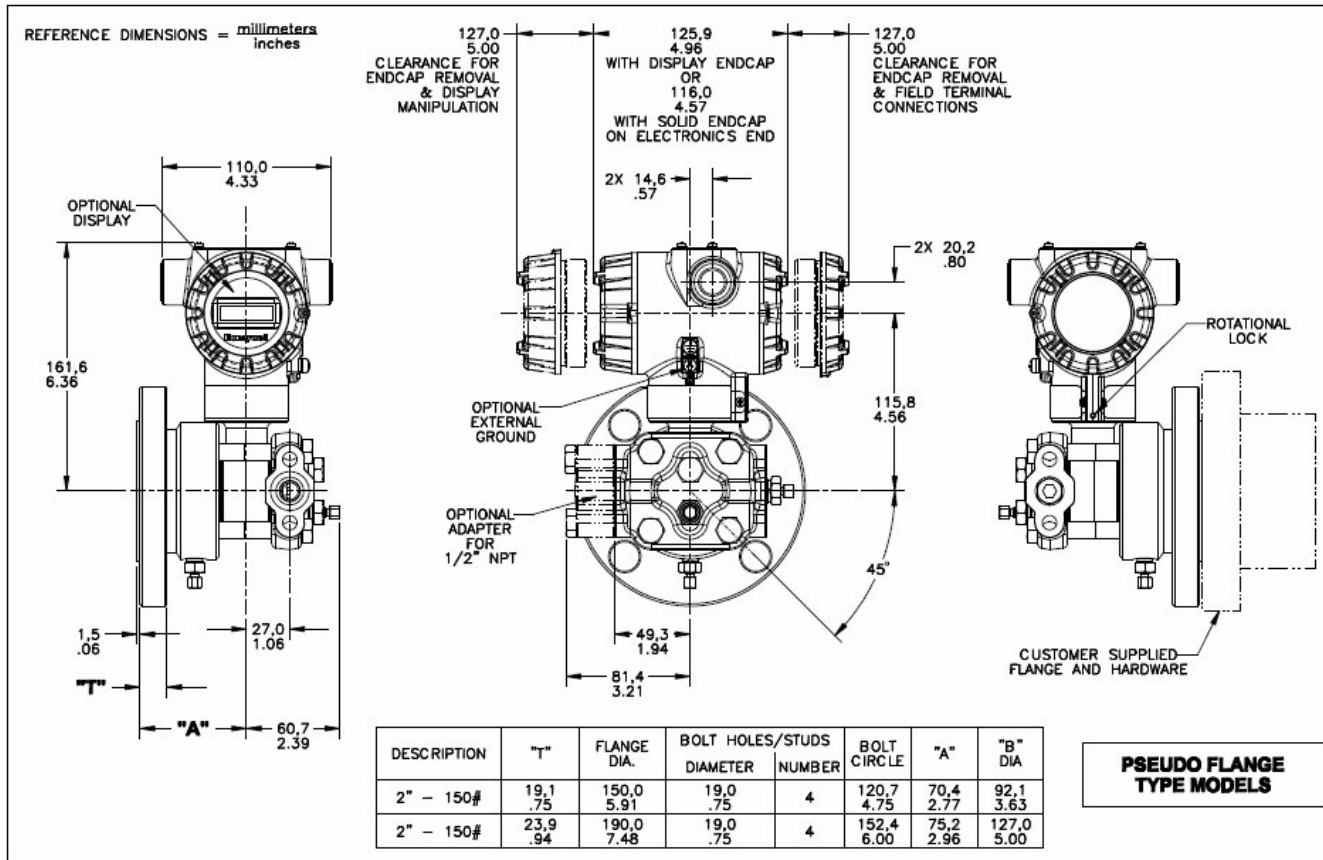
Figure 6 – Typical mounting dimensions for pseudo flange type models STF72F, STF73F, and STF74F.
