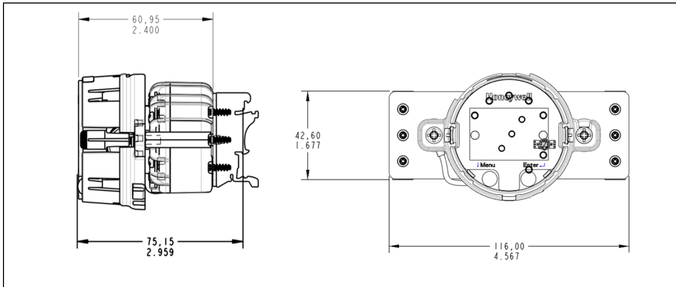
Figure 6: DIN Rail Mounting Dimensions (With Display)
