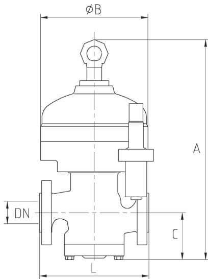
Dimensional Sketch (Example) HON R100
