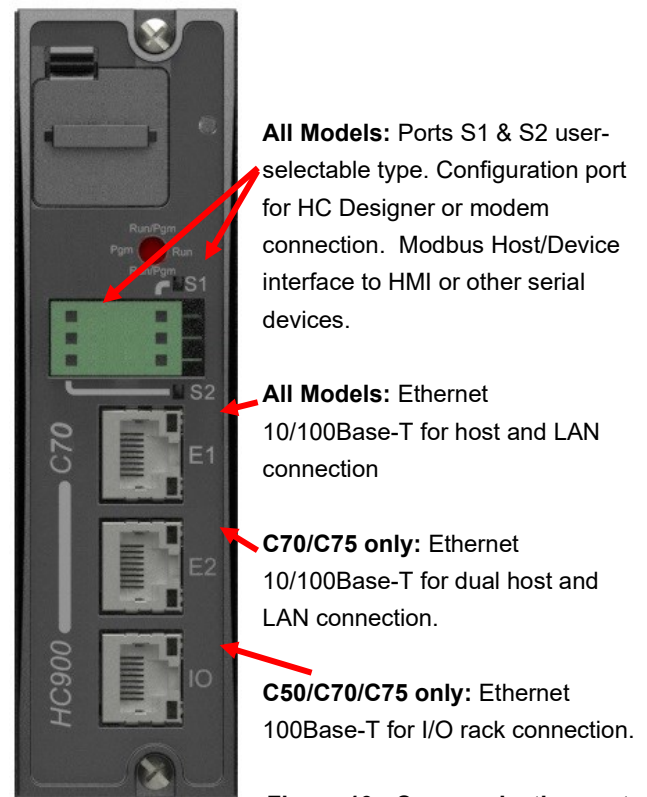
Figure 10 - Communication ports
