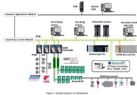
Figure 1. Sample Experion LX architecture
