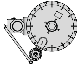
Assembly Position "B4.5"
