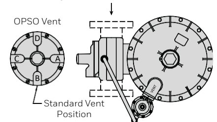
Assembly Position "C4.5"
