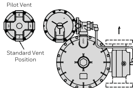
Valve Head Position "D"
