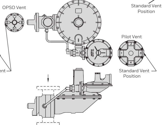
Valve Head Position "D"
