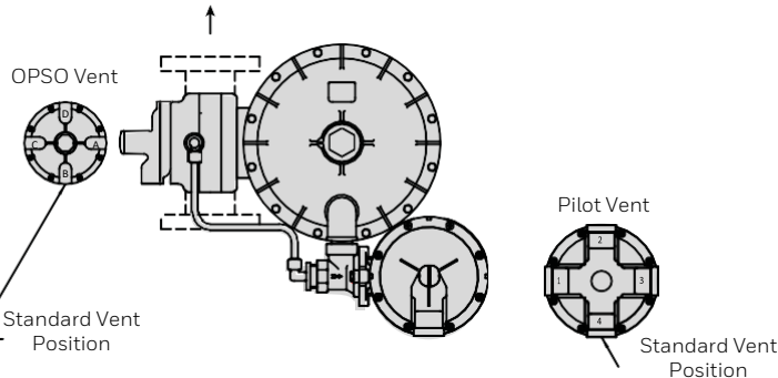
Valve Head Position "D"
