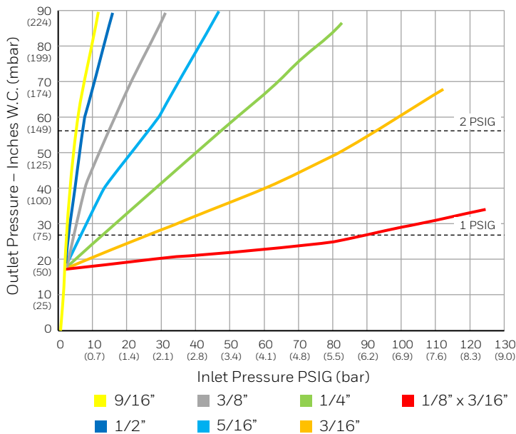
1" Screen Vent – No Vent Pipe Set Pressure 7" W.C.
