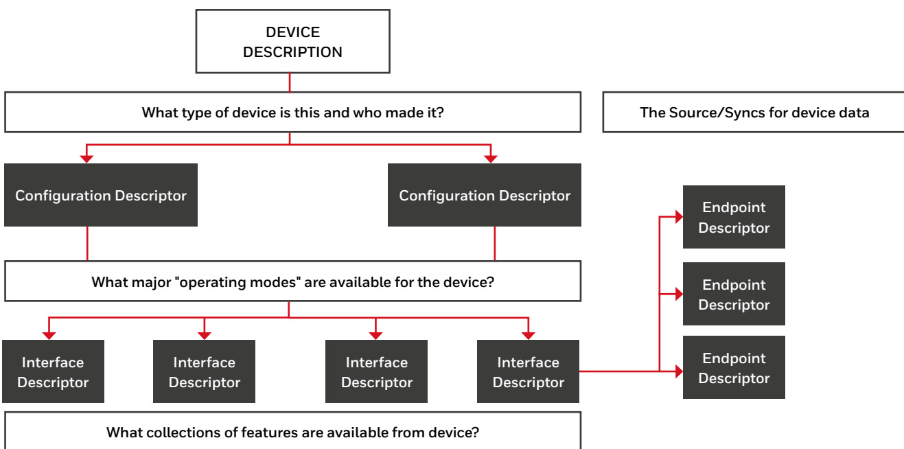
Figure 2 - Each USB device describes and identifies itself by sending a series of descriptors to the host...meaning it can lie...
