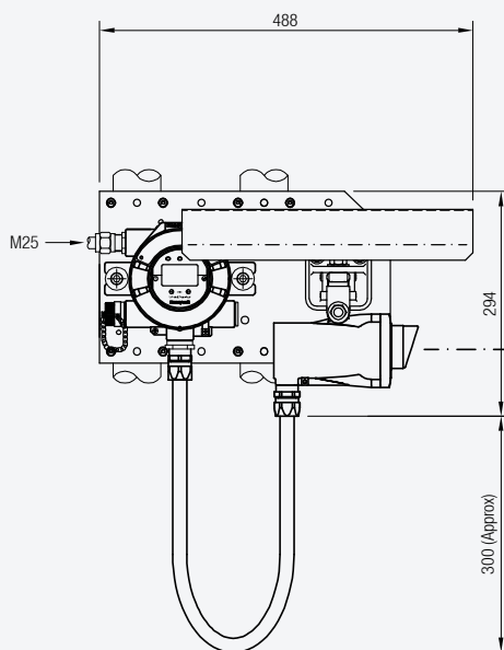
Pipe Mounted
