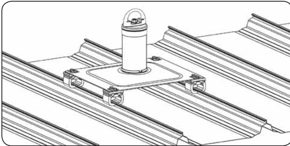
Fig. 4c - Completely Installed
