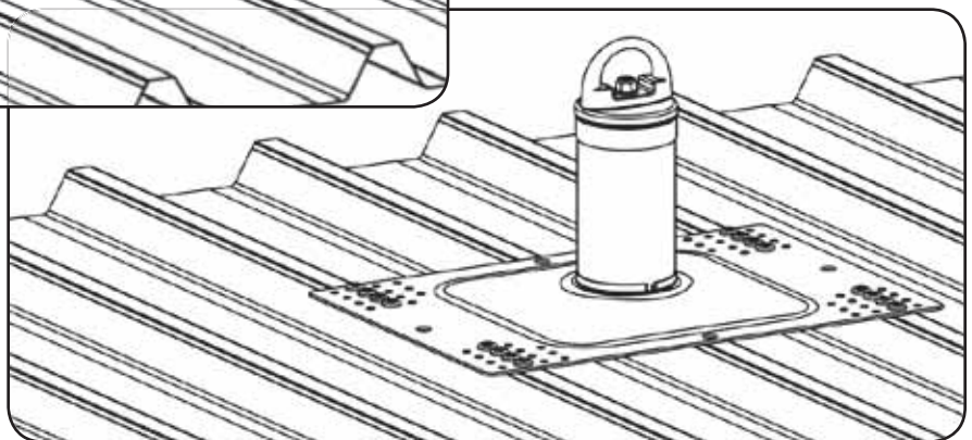
Fig. 8c - Completely Installed
