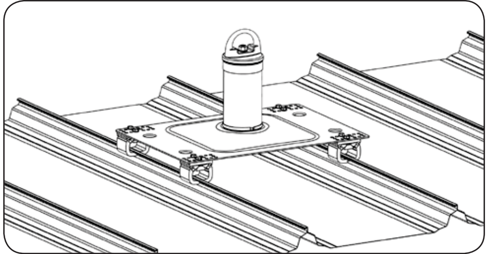
Fig. 5c - Completely Installed
