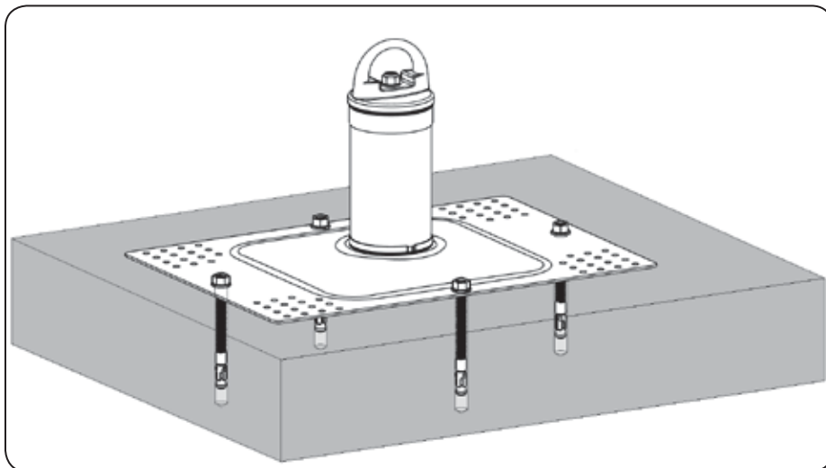
Fig. 11c - Completely Installed
