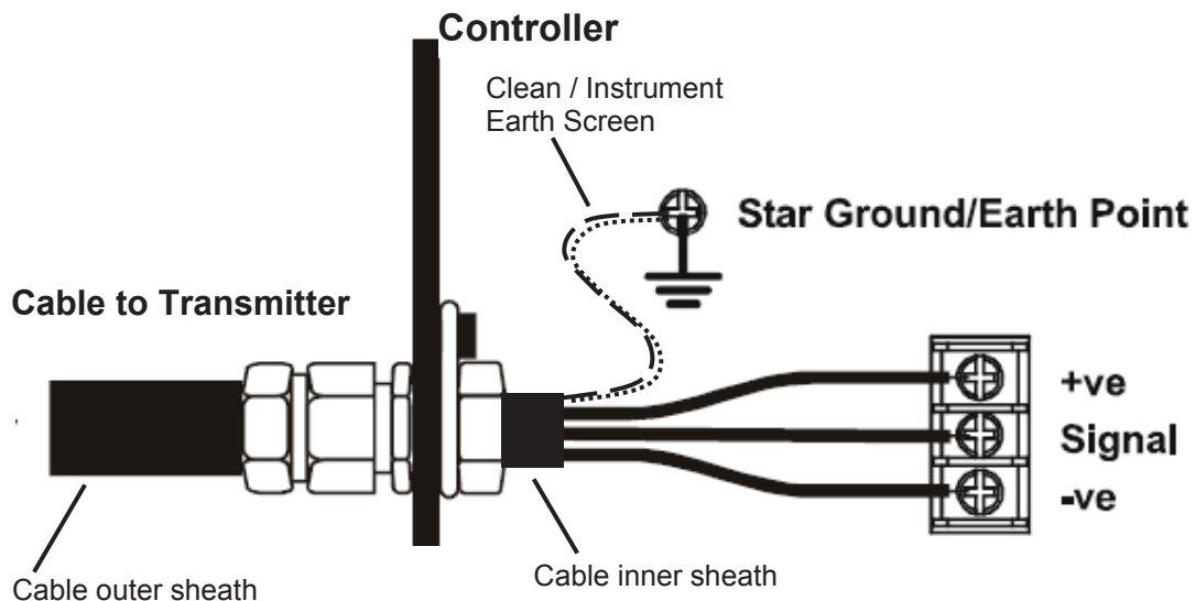
Diagram 10: Controller Grounding
