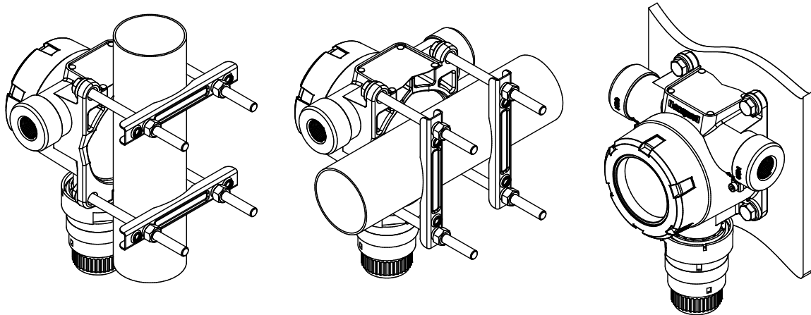
Diagram 5: Mounting arrangements
