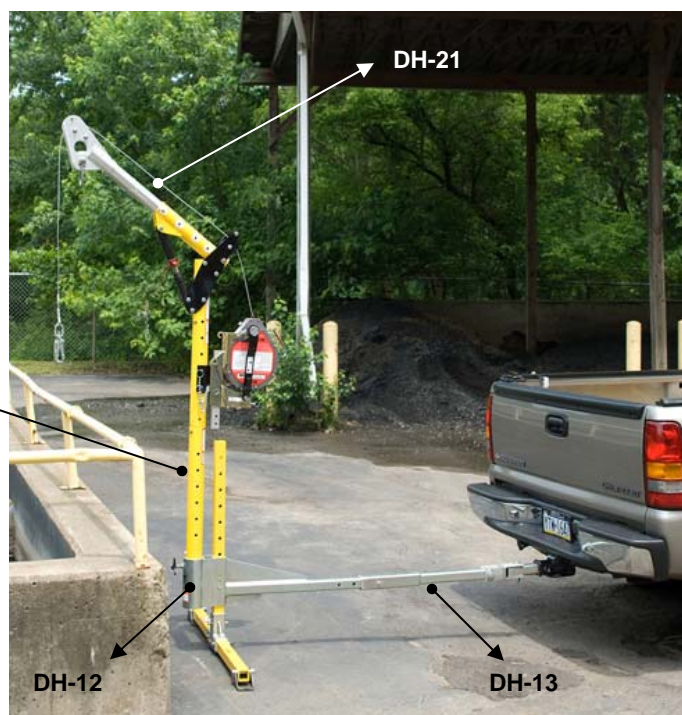
2-ft. Vehicle Hitch Mount Extension (DH-13) installed between Vehicle Hitch Mount Sleeve (DH-12) and attendant vehicle:
