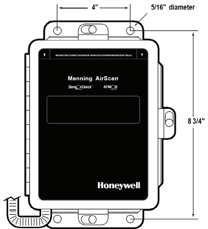
Figure 1. Mounting Dimensions
