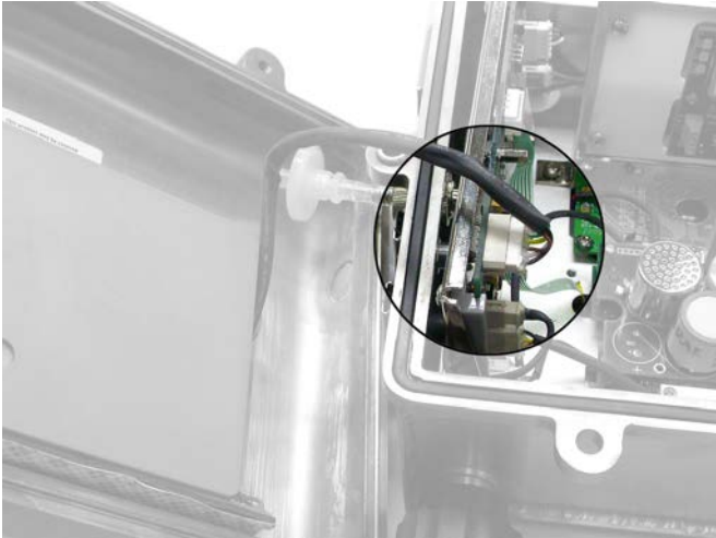
Figure 7-3 Battery connection
