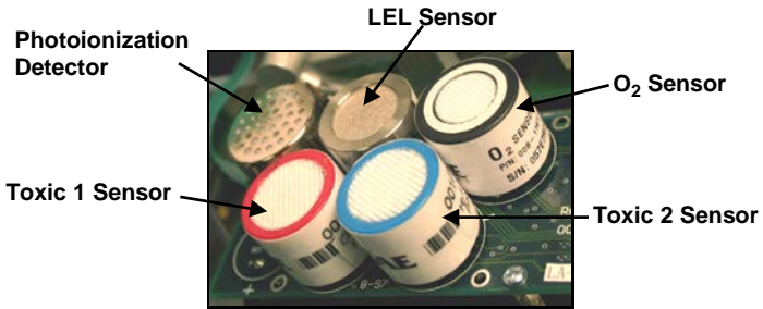
Figure 7-5 Sensor locations
