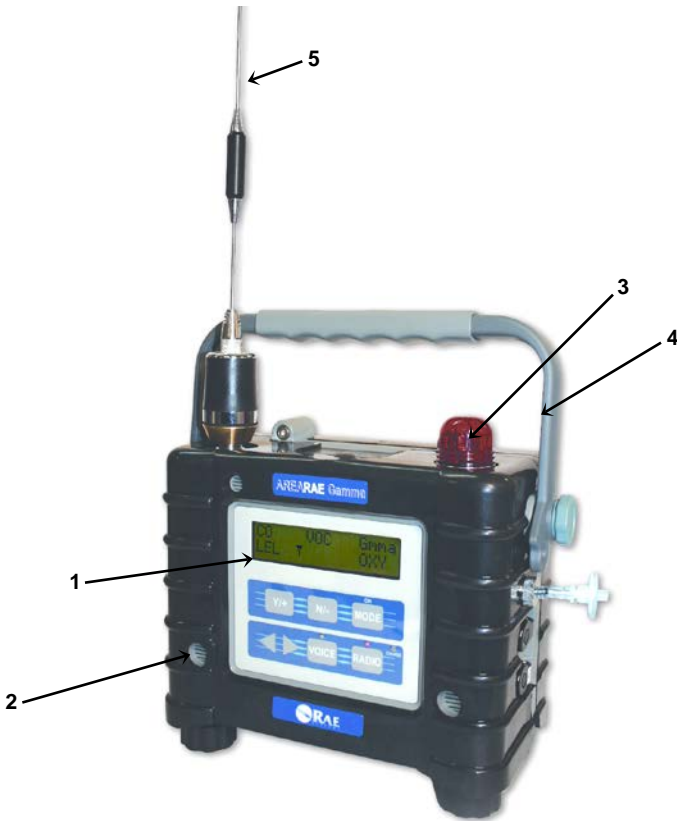
Figure 2-1 Front View: Main Components
