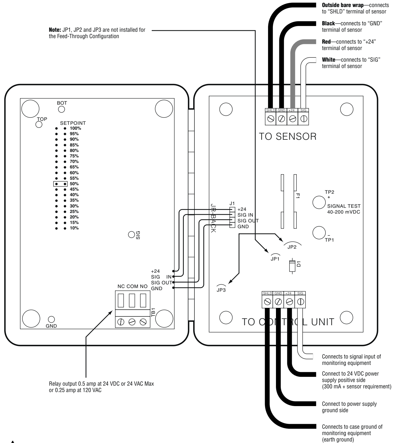
Figure 2: Wiring diagram for the Manning GM-JR Gas Monitoring Alarm System – Feed-Through Configuration
