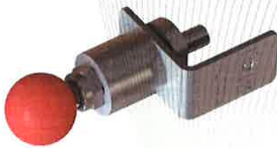
Fig.11: End stop, type: climbing lock for steel / stainless steel ladders and guide rail made of steel / stainless steel / aluminium
