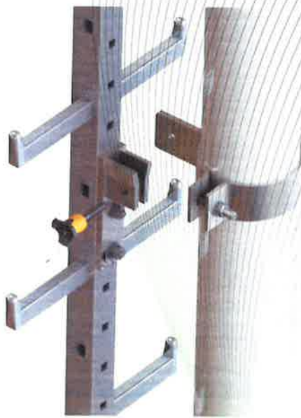
Fig. 25: Holding system for hook ladders for mounting from below
