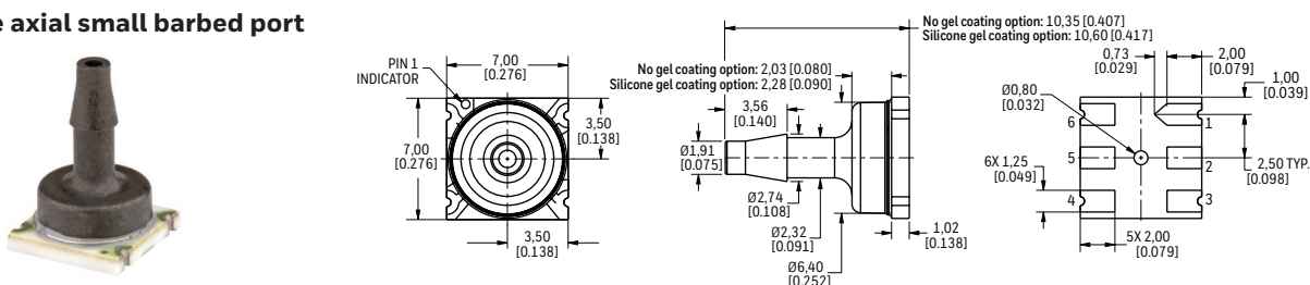
FIGURE 3. LEADLESS SMT PACKAGE DIMENSIONAL DRAWINGS (FOR REFERENCE ONLY: MM [IN].)
