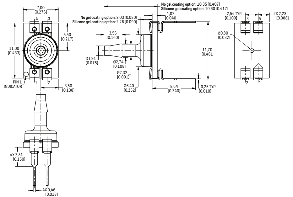
FIGURE 1. DIP PACKAGE DIMENSIONAL DRAWINGS (FOR REFERENCE ONLY: MM [IN].)
