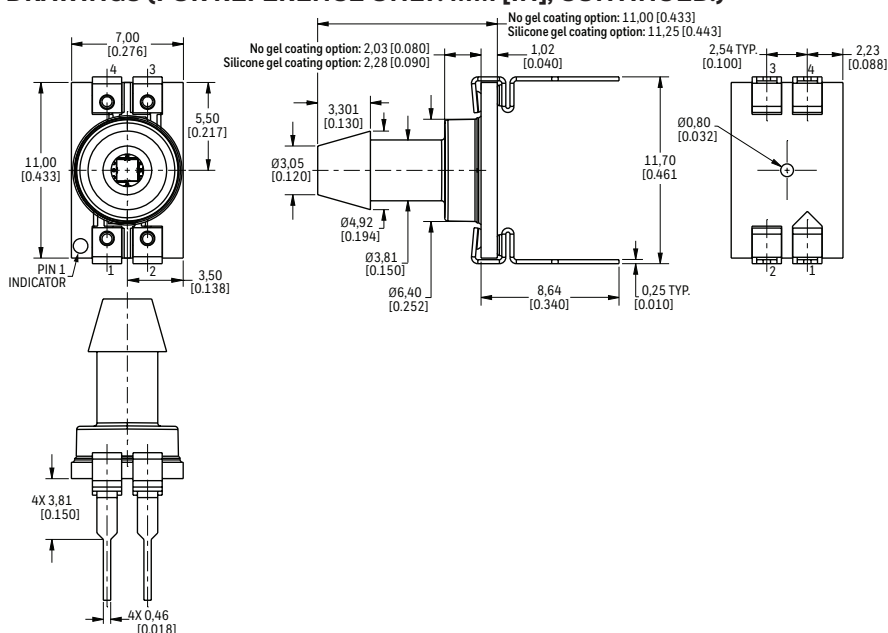
FIGURE 1. DIP PACKAGE DIMENSIONAL DRAWINGS (FOR REFERENCE ONLY: MM [IN], CONTINUED.)
