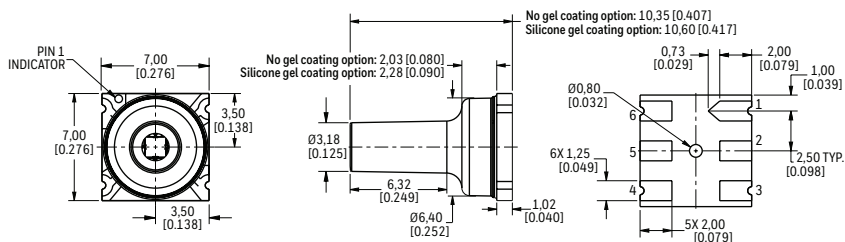
FIGURE 3. LEADLESS SMT PACKAGE DIMENSIONAL DRAWINGS (FOR REFERENCE ONLY: MM [IN], CONTINUED.)
