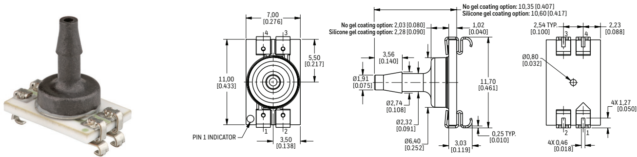
FIGURE 2. SMT PACKAGE DIMENSIONAL DRAWINGS (FOR REFERENCE ONLY: MM [IN].)
