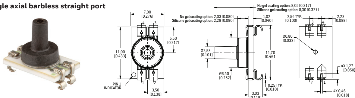
FIGURE 2. SMT PACKAGE DIMENSIONAL DRAWINGS (FOR REFERENCE ONLY: MM [IN], CONTINUED.)
