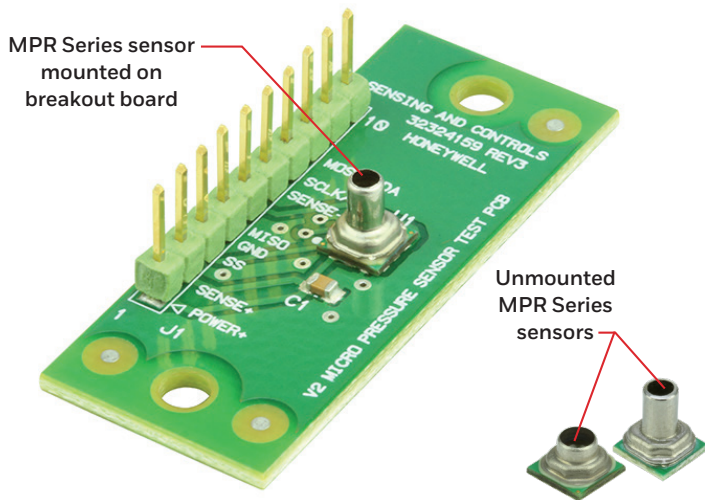
Figure 7 . MPR Series Breakout Board
