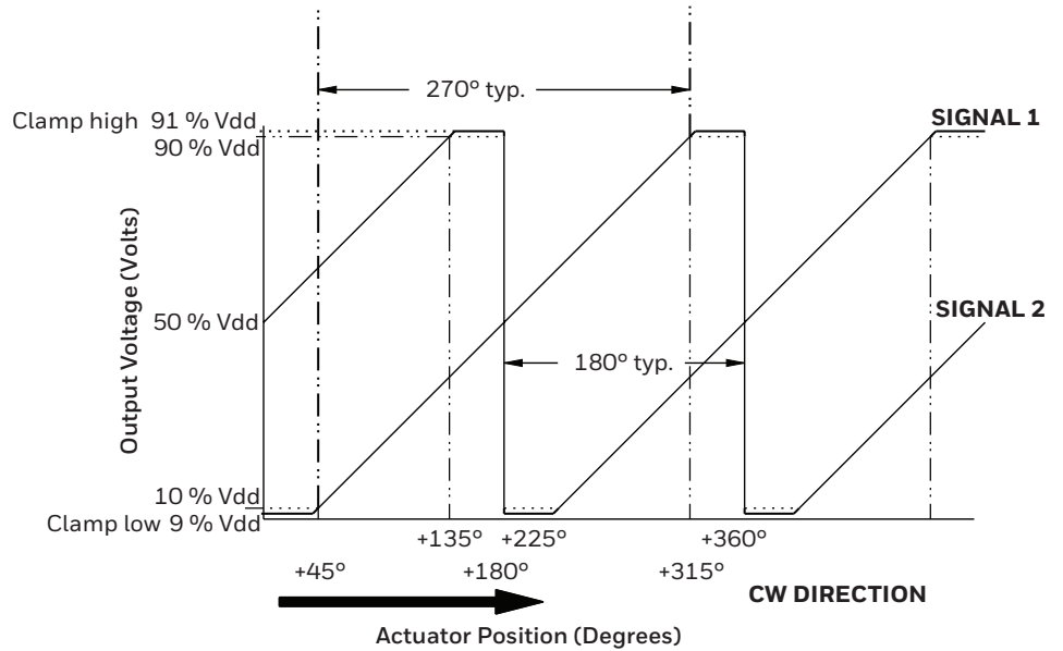
Figure 1. Characteristic Curve
