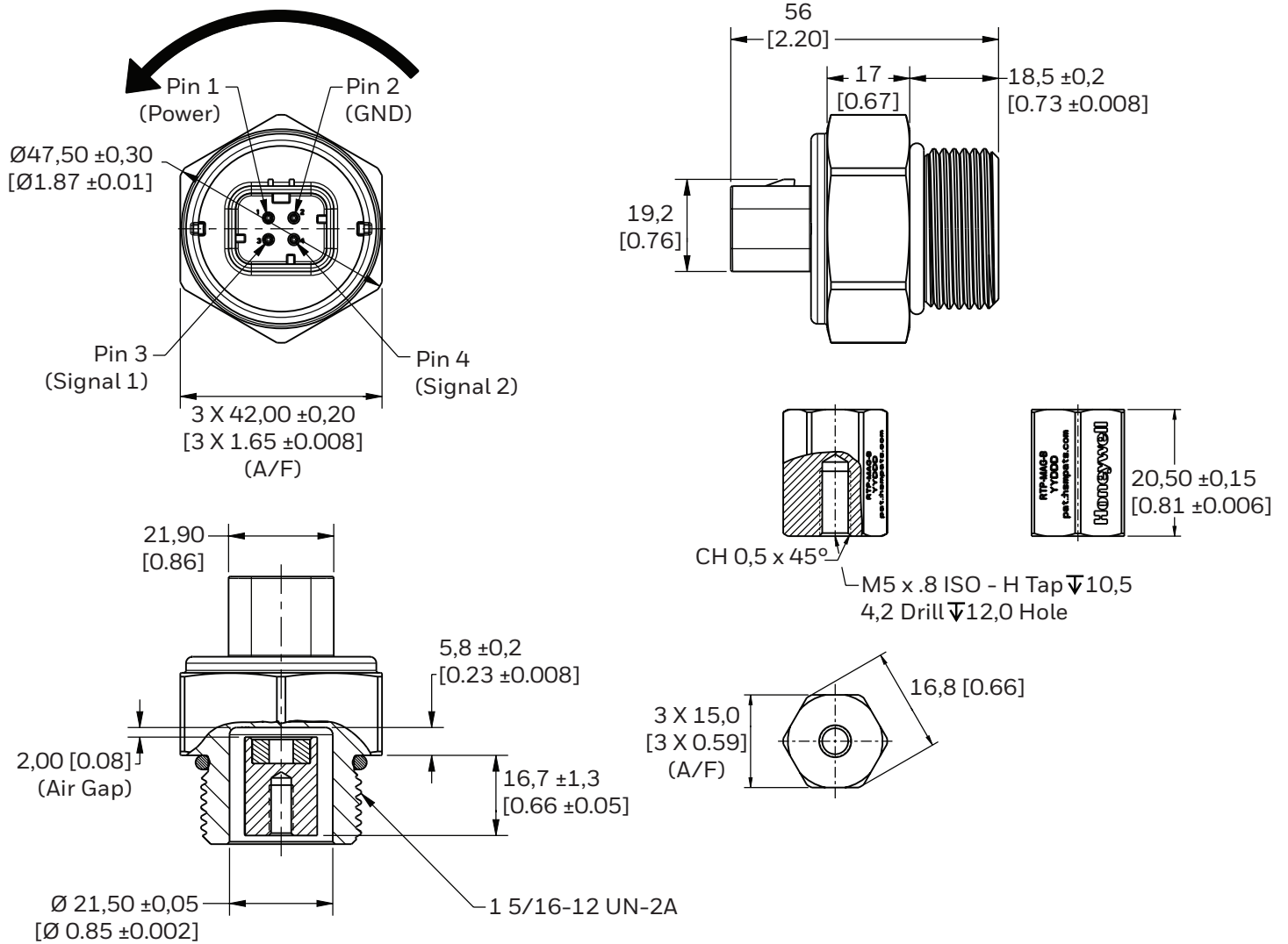
Figure 2. Dimensional Drawing
