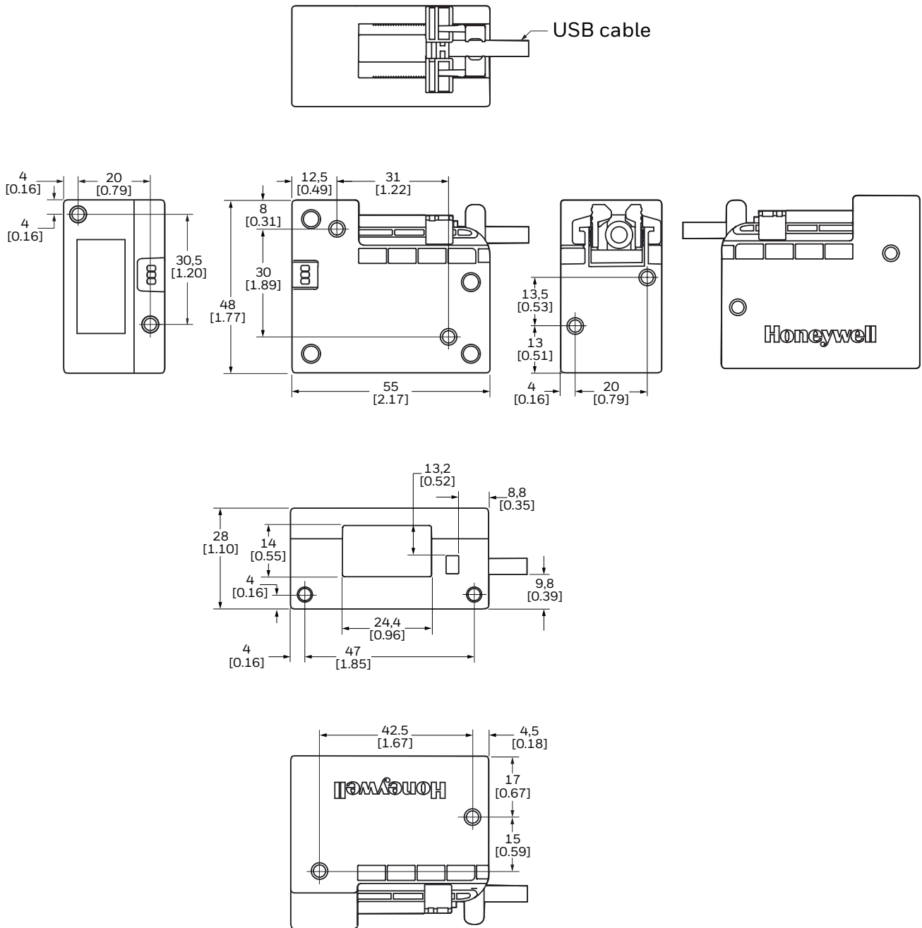
Figure 5. Mounting and Dimensional Drawing (For reference only: mm/[in].)
