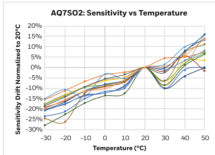
Figure 6. Sensitivity vs. Temperature
