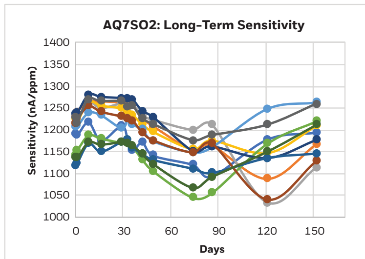
Figure 9. Long-Term Sensitivity Drift
