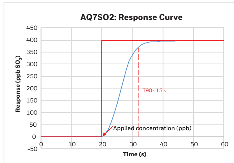
Figure 2. AQ7SO2 Gas Response Profile
