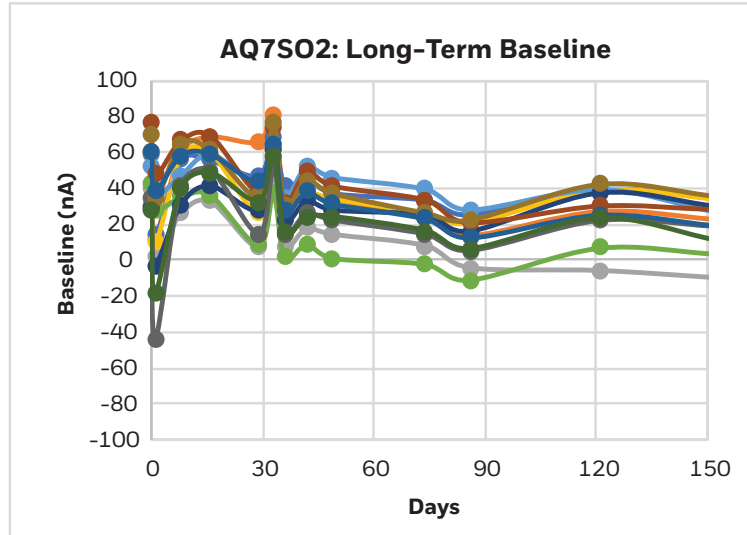
Figure 8. Long-Term Baseline Drift
