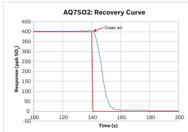
Figure 3. AQ7SO2 Gas Recovery Profile
