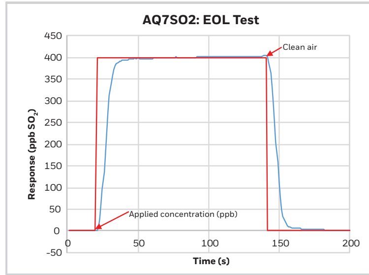
Figure 2. AQ7SO2 Gas Response Profile
