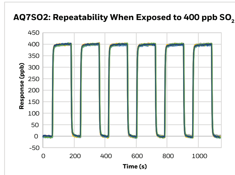
Figure 11. Repeatability of AQ7SO2 Sensor response to 400 ppb SO 2
