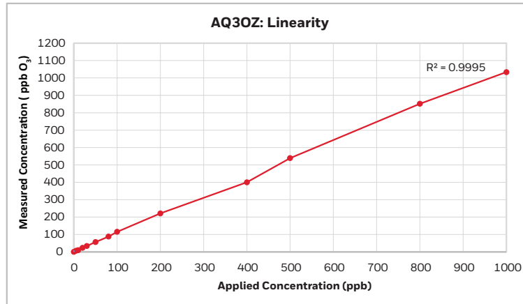
Figure 4. Output Linearity from 0 ppb to 1000 ppb
