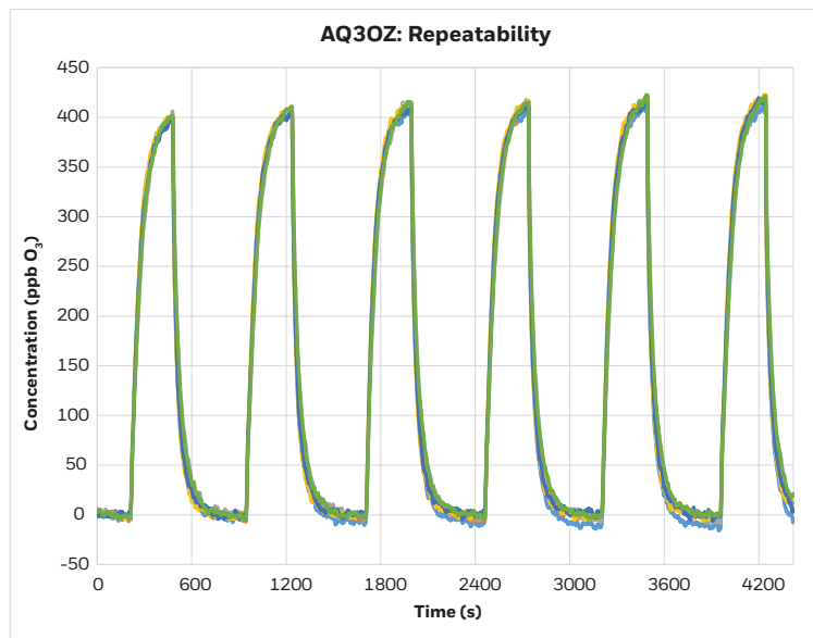
Figure 9. Repeatability of AQ30Z Sensor response to 400 ppb O 3
