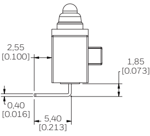
TYPE 30 TERMINALS WITH TYPE 3 PILLARS
