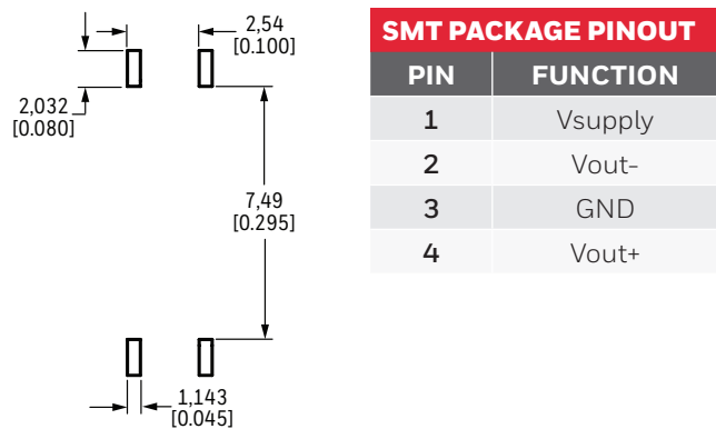
Figure 5. Leadless SMT Package Dimensional Drawings (For reference only: mm [in].)
