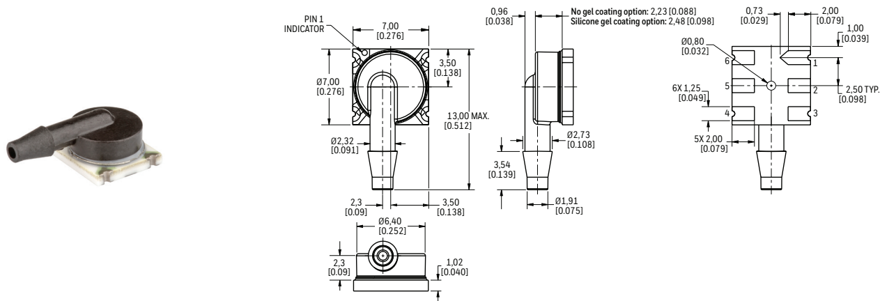
Figure 5. Leadless SMT Package Dimensional Drawings (For reference only: mm [in], continued.)
