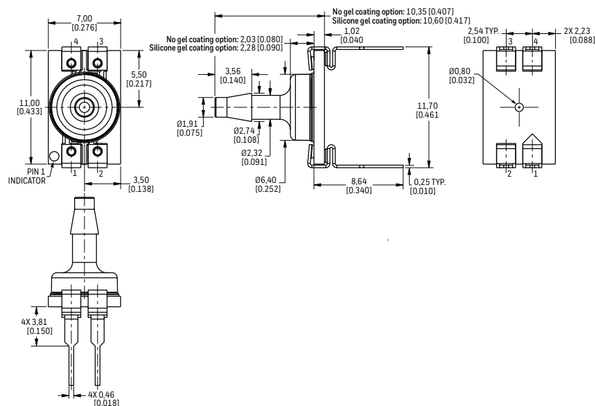
Figure 3. DIP Package Dimensional Drawings (For reference only: mm [in.]
