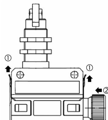
Figure 5 – Assemble switch
