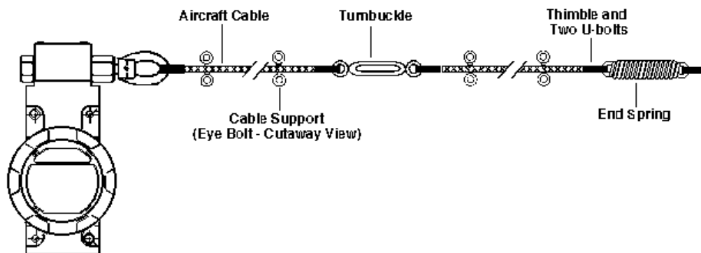
Figure 3: Switch with Turnbuckle and Endspring
