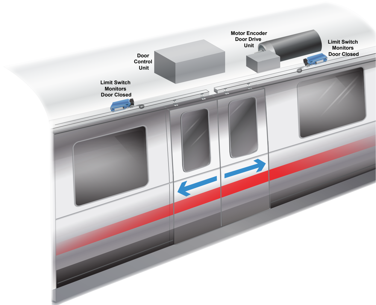
Figure 2. MICRO SWITCH NCG Series in Rail Door Applications
