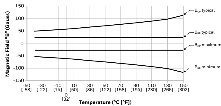
Figure 3. Transfer Characteristics
