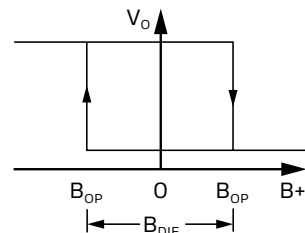
Figure 3. Transfer Characteristics
