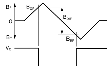
Figure 4. Transfer Characteristics Definition
