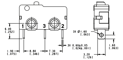
Terminal Type 20 - Straight PCB
