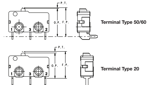
Operate Point References for PCB Terminals
