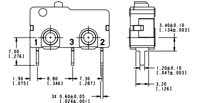
Terminal Type 70 - Long Solder
