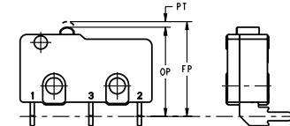
Operate Point References for PCB Terminals
