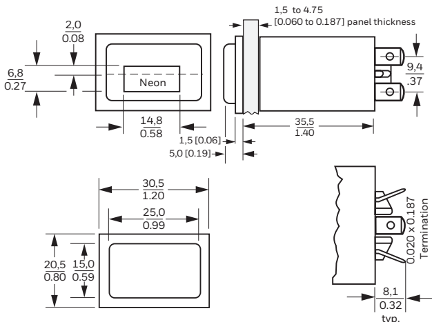
Figure 9. AML32 Series Dimensions mm [in] or mm/in
