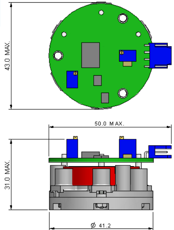
All dimensions in mm All tolerances ±0.15 mm unless otherwise stated
