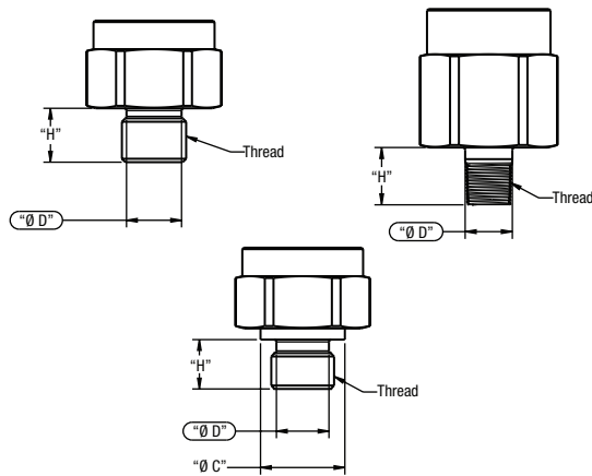
Figure 7. HP Series Pressure Port Dimensions
