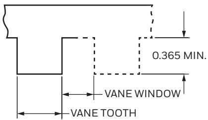
FIGURE 3. VANE DIMENSIONS (FOR REFERENCE ONLY (IN))
